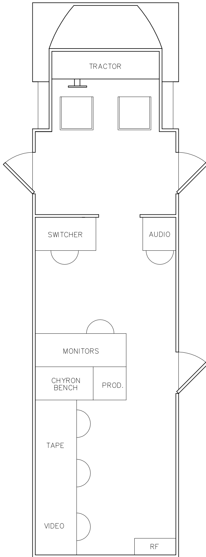
MILLENNIUM-1 FLOOR PLAN
